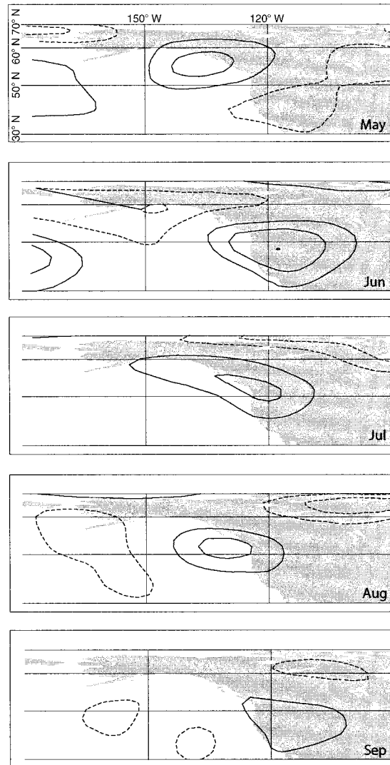
FIG. 2. The 500-hPa height anomaly field projected onto the regional burned area index (BAI), May–September. This pattern describes the atmospheric variability associated with a one-standard-deviation perturbation in BAI. The contour interval is 5 m, with positive anomalies indicated by a solid contour, negative anomalies by a dashed contour, and the zero line not shown. Cross-hatched regions indicate that the correlation at that gridpoint is significant at the 95% confidence level.
