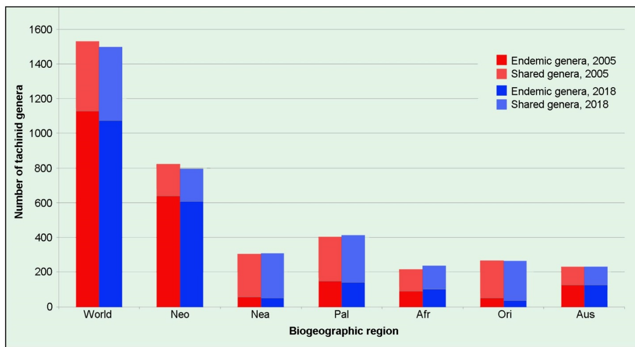
Figure 2. Number of tachinid genera recognized in the world and per biogeographic region in 2005 and 2018, with levels of endemism.
