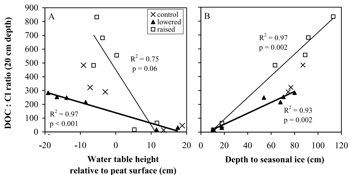
Figure 6. Pore water [DOC:Cl] concentrations (a) measured at 20 cm depth declined with increasing water table height and (b) increased as depth to seasonal ice increased across the water table treatments.
