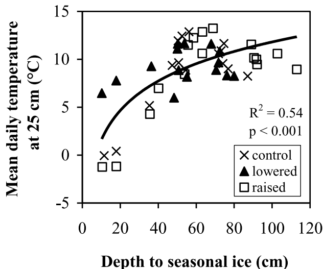
Figure 2. Mean daily peat temperatures (25 cm) increased as the depth to seasonal ice increased with the progression of the growing season. Coefficients describing the natural logarithmic trend are \beta_0 = -8.66 \pm 2.46 , \beta_1 = 4.44 \pm 0.62 .
