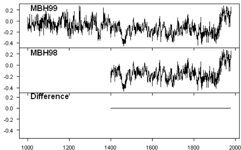
Figure 11: Top panel: MBH99 hockey stick. Middle panel: MBH98 hockey stick. Bottom panel: differences.
