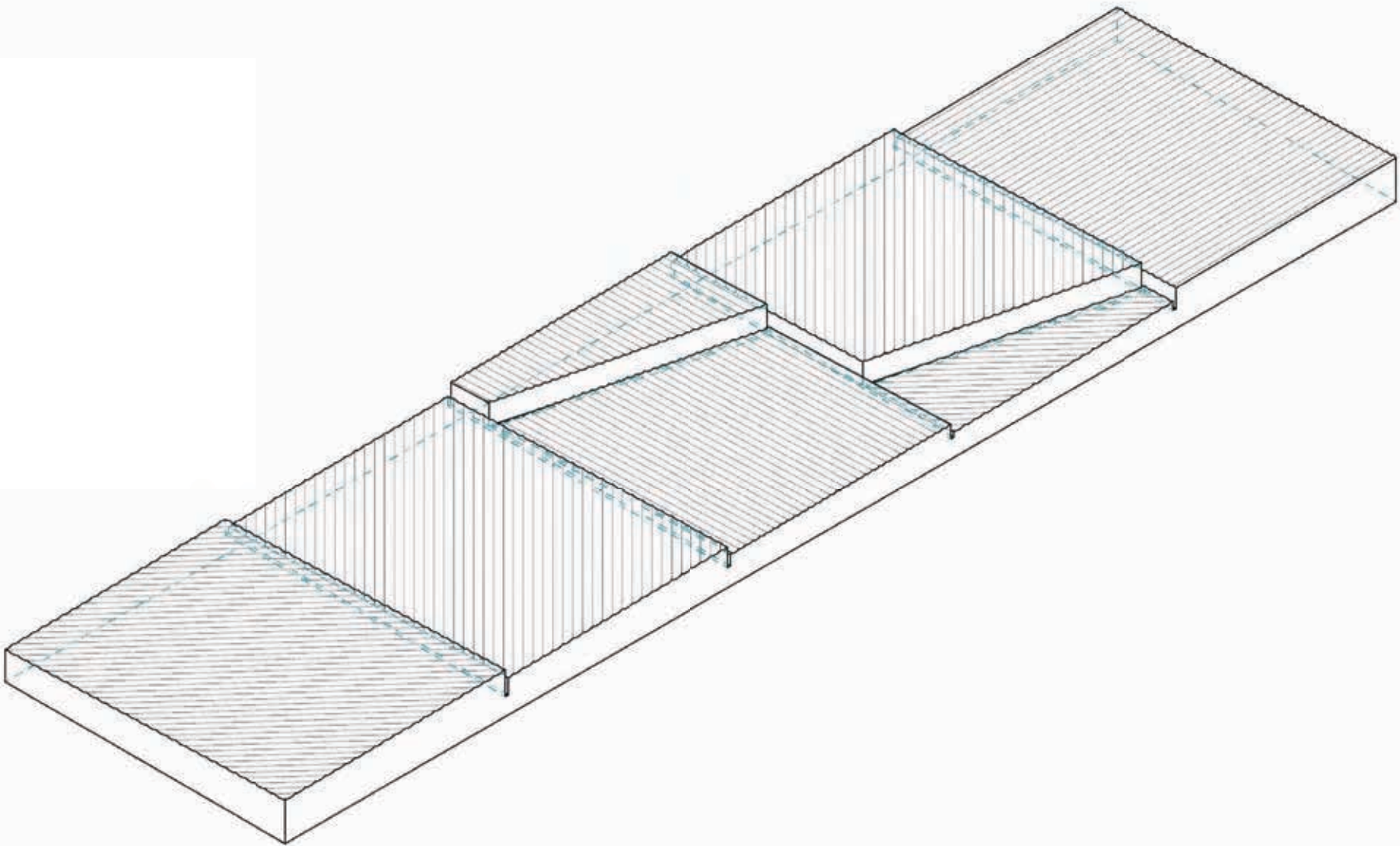
Typical Precast Panel: 5 Divisions × 1200mm; Panel Qty.: 16 Panels
